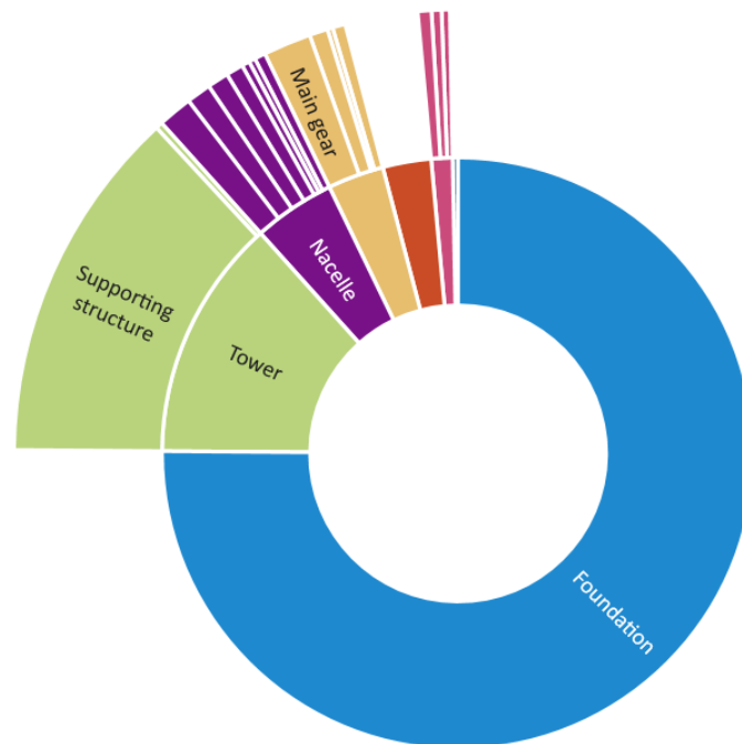
Figure 5: Composition breakdown by mass for the Delta4000 turbine
