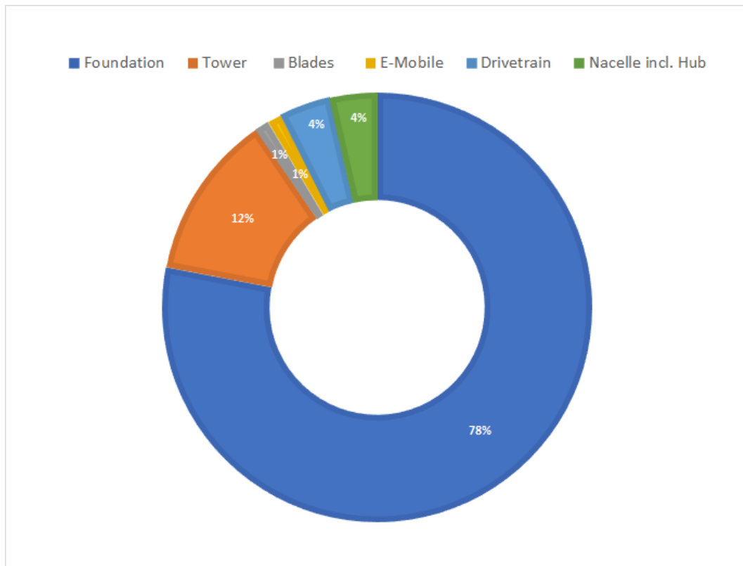
Figure 4: Composition breakdown by mass for the Delta4000 turbine
